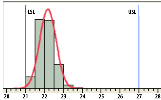
Gain @ 30\text{ GHz} ( P_{in} = -20\text{ dBm} ), Mean = 22.09\text{ dB} , LSL = 21\text{ dB} , USL = 27\text{ dB}
