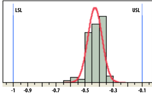
V_g @ V_{dd} = 6\text{ V} , I_{dq} = 3\text{ A} ( P_{in} = -20\text{ dBm} ), Mean = -0.42\text{ V} , LSL = -1\text{ V} , USL = -0.1\text{ V}
