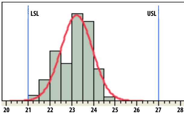
Gain @ 29.5\text{ GHz} ( P_{in} = -20\text{ dBm} ), Mean = 23.37\text{ dB} , LSL = 21\text{ dB} , USL = 27\text{ dB}
