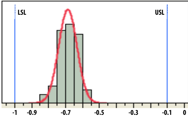
V_g @ V_{dd} = 6\text{ V} , I_{dq} = 3\text{ A} ( P_{in} = 17\text{ dBm} ), Mean = -0.68\text{ V} , LSL = -1\text{ V} , USL = -0.1\text{ V}
