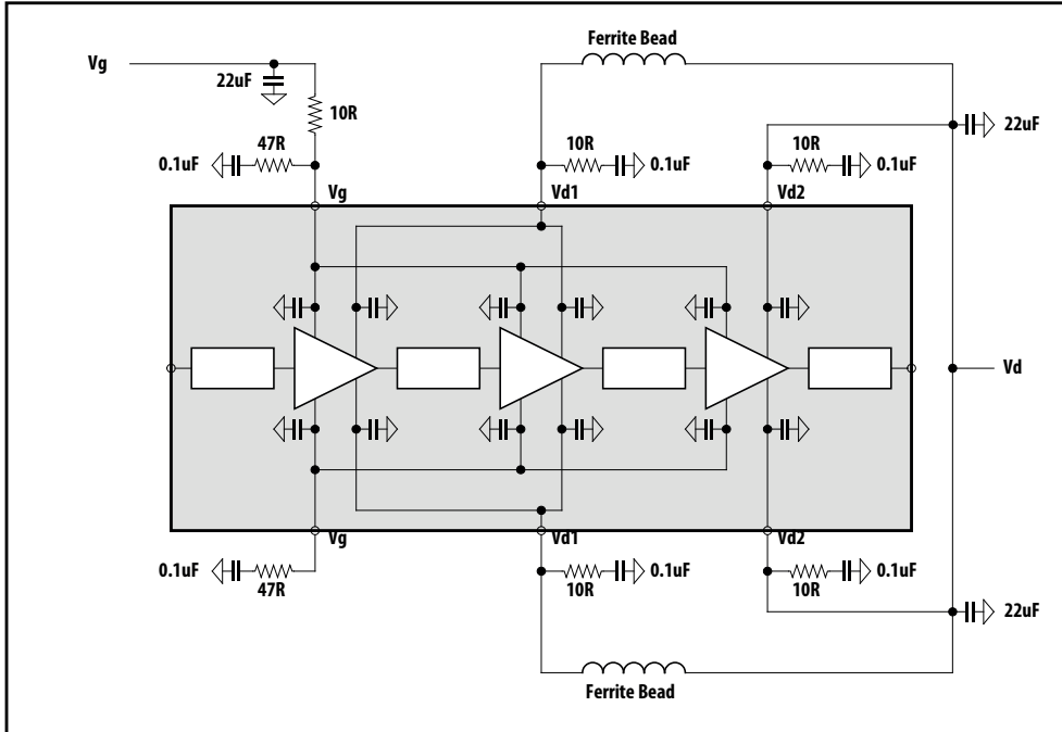
Figure 19. Application Circuit
